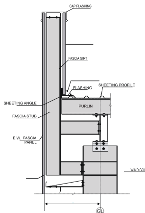
Projected Curved Fascia
