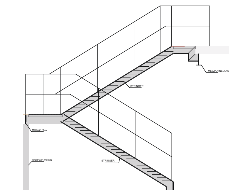
ELEVATION- Double Flight Staircase
