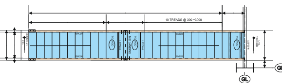
Staircase Plan
