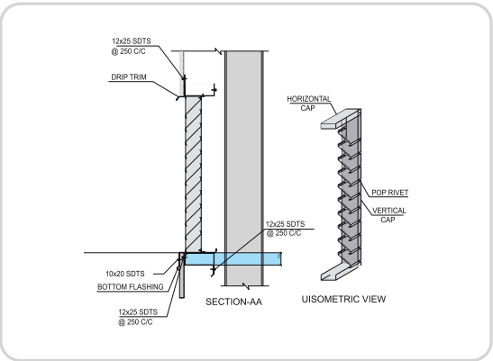
S Type Fixed Louvers
