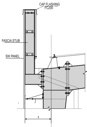
Flush Fascia Side wall Detail
