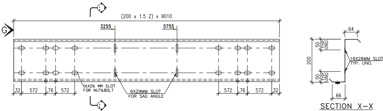
200 Z SECTION COMMON DETAIL
