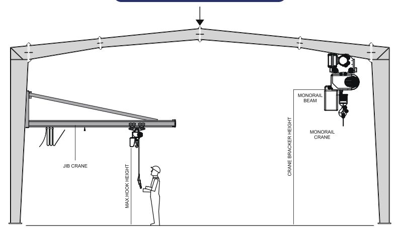
JIB Crane
