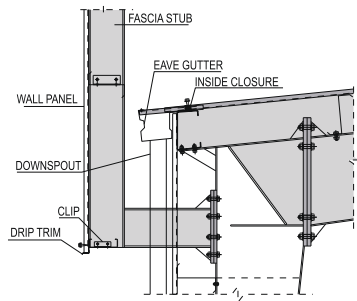
Projected Fascia with Eave Gutter
