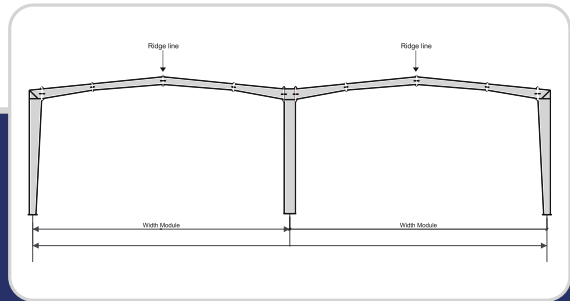
Multi Gable (MG)
