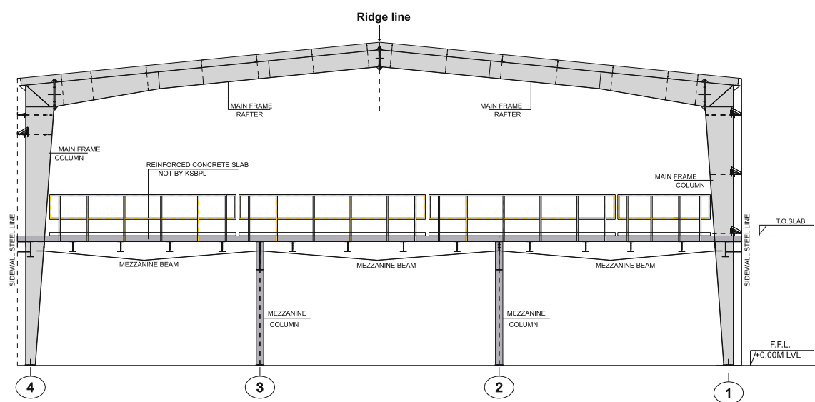
Mezzanine Framing Elevation
