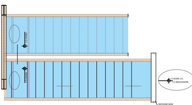
Staircase Plan
