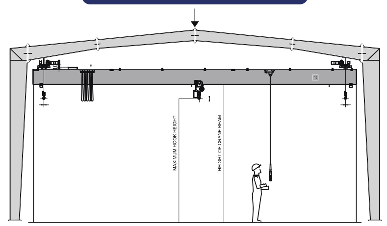
Under Slung Crane
