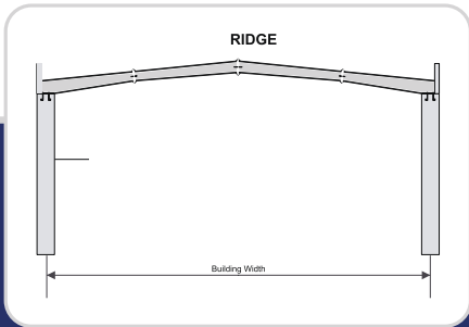
Rafter System
