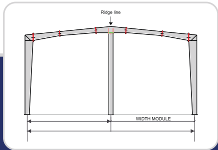
Multi Span (TCMS-1)
