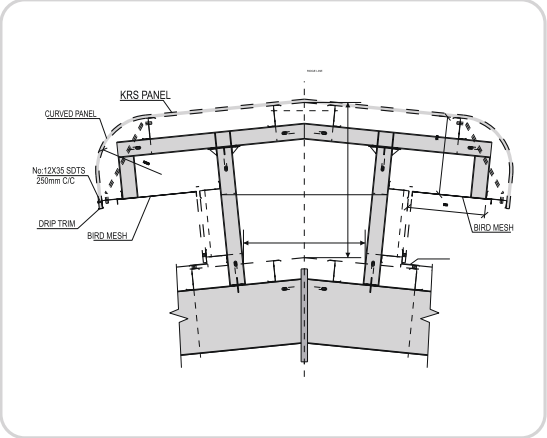
Ridge Vent
