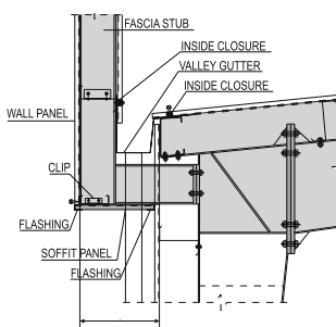
Projected Fascia Side wall Detail
