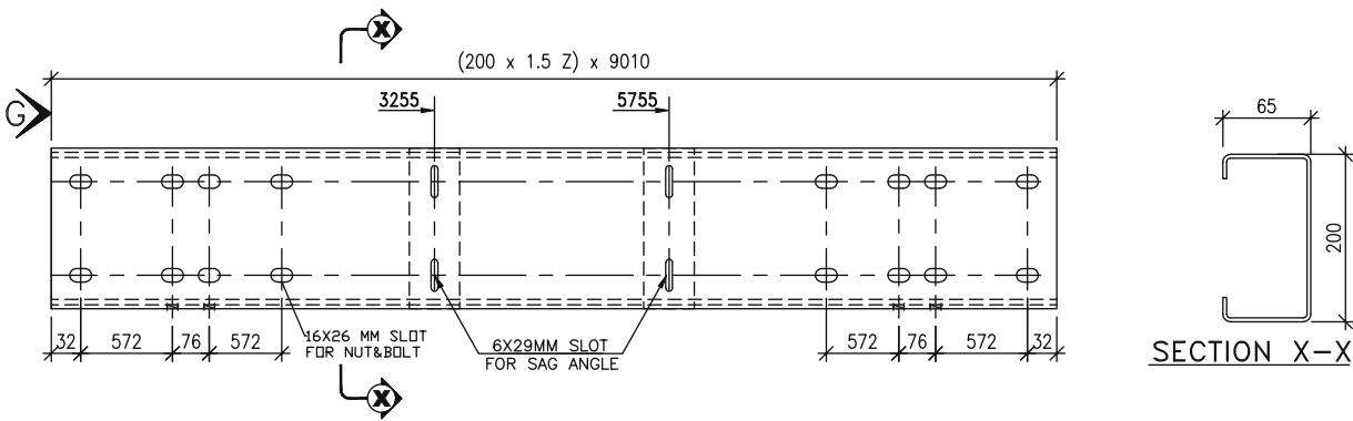
200C SECTION COMMON DETAIL
